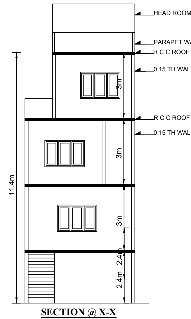
SECTION @ X-X
