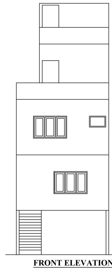
FRONT ELEVATION
